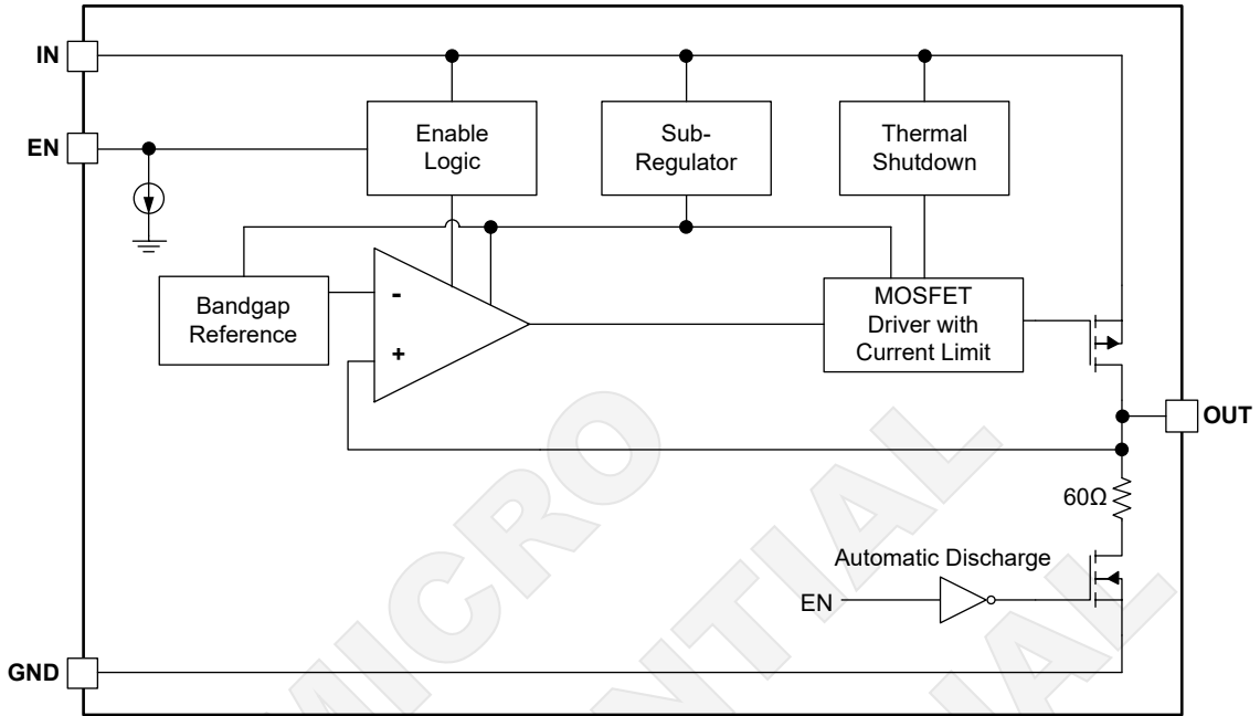
Figure 2. Block Diagram
