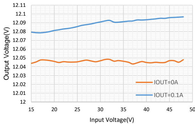
Figure 6. Line Regulation
