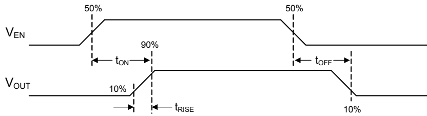
Figure 3. SGM2581A/C/E/G//K Switch Turn-On and Turn-Off Delay Times
