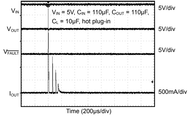
Capacitance Load Inrush Response (SGM2581A/B/G)
