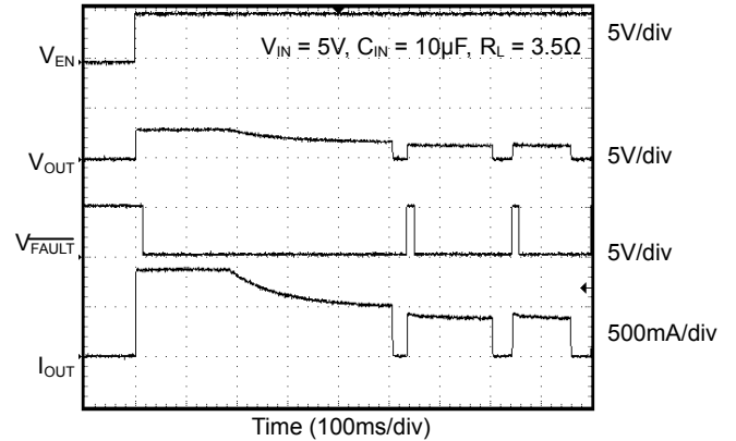
Thermal Shutdown Response (SGM2581A/G)
