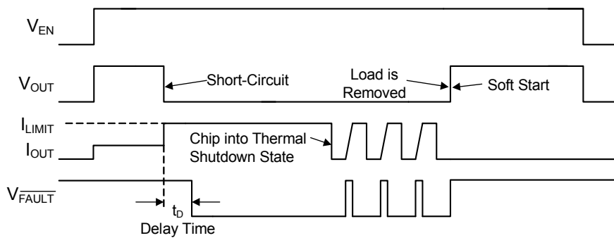
Figure 5. SGM2581A/C/E/G//K Fault Timing: Output Reset by Removing Load
