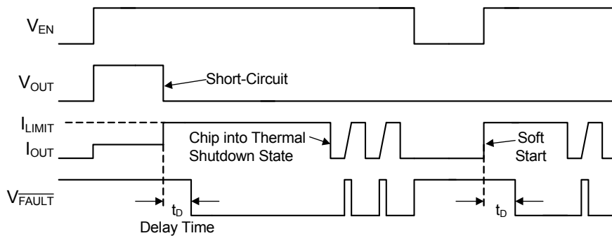
Figure 4. SGM2581A/C/E/G//K Fault Timing: Output Reset by Toggling EN
