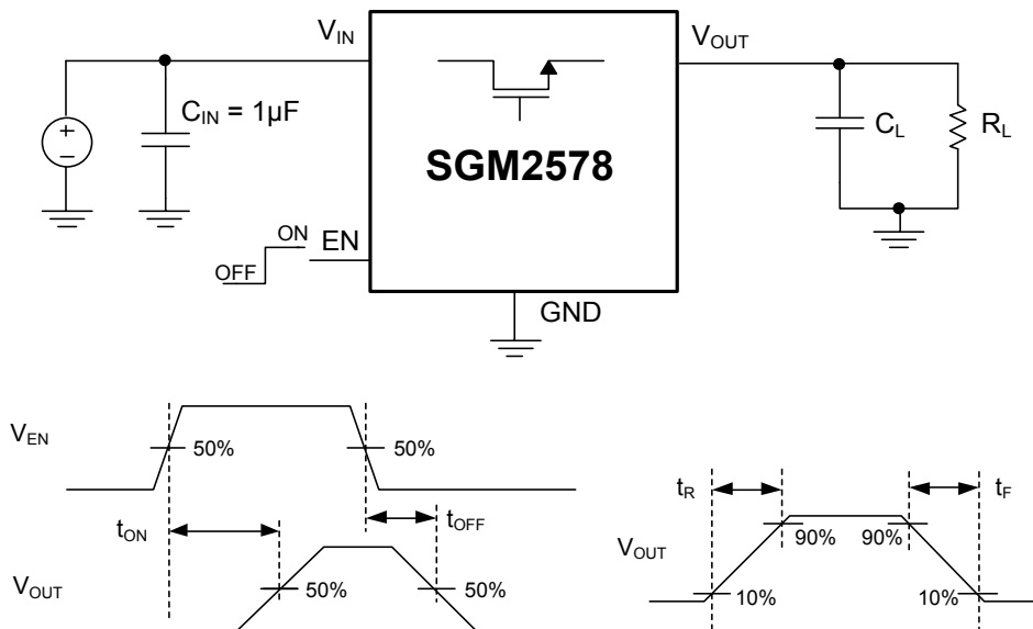
Figure 3. Test Circuit and t_{ON}/t_{OFF} Waveforms
