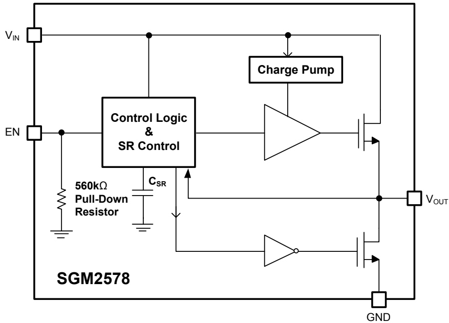
Figure 2. Block Diagram
