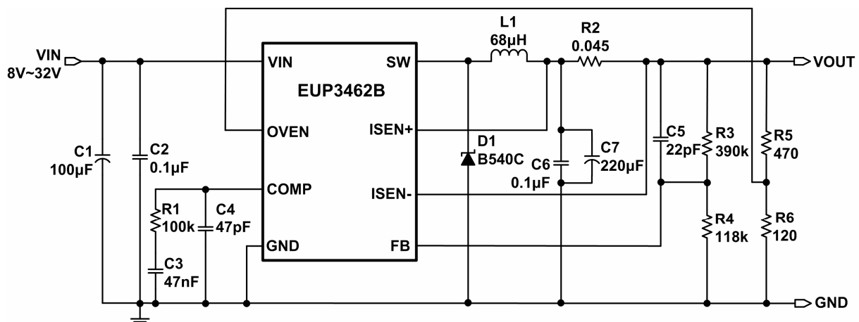
Figure 1. Application Circuit
