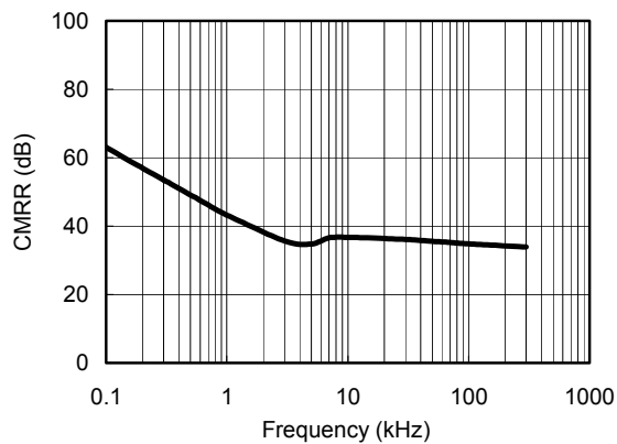
CMRR vs. Frequency at +2.5V
