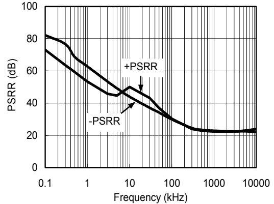
PSRR vs. Frequency at ±1.25V
