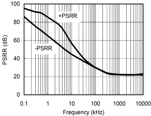
PSRR vs. Frequency at ±2.5V
