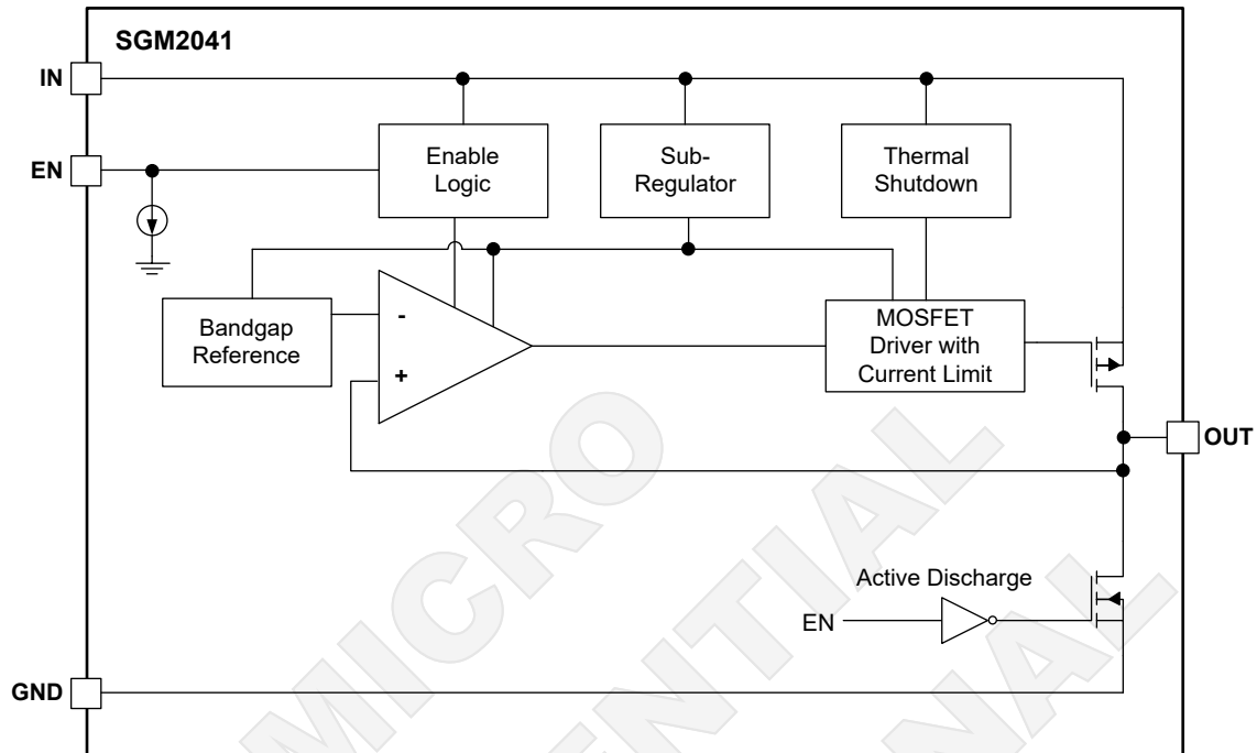
Figure 2. Block Diagram
