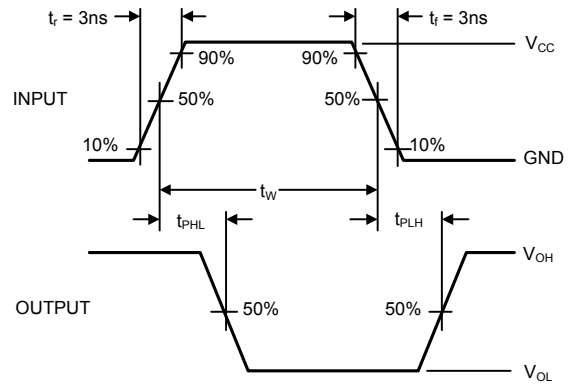
Figure 2. AC Waveforms
