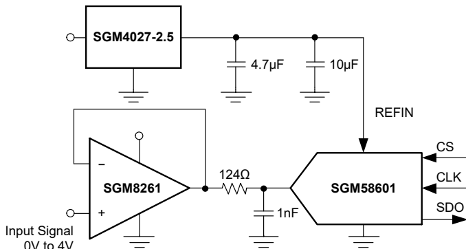
Figure 5. Data Acquisition System with SGM4027
