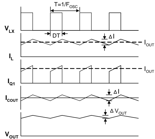
Figure 1. Converter Waveforms
