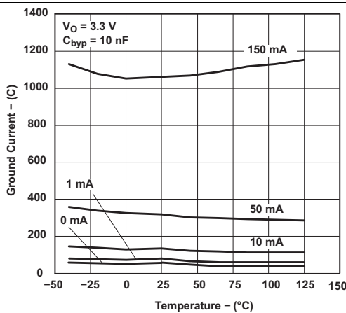
Figure 17. Ground-pin Current vs Temperature
