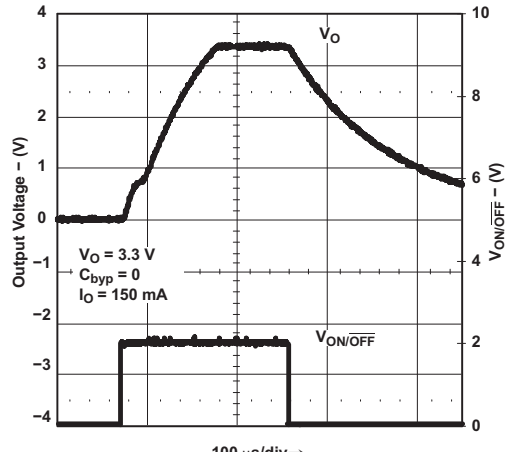
Figure 28. Turn-on Time
