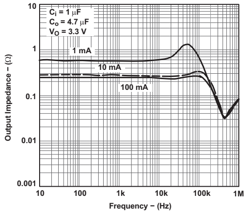
Figure 13. Output Impedance vs Frequency
