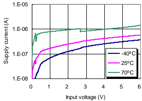
Detector threshold=2.7V
