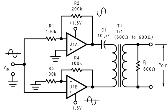
Figure 43. Differential Driver
