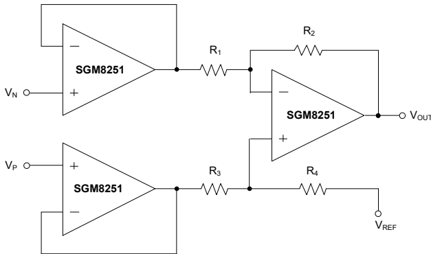
Figure 5. Instrumentation Amplifier
