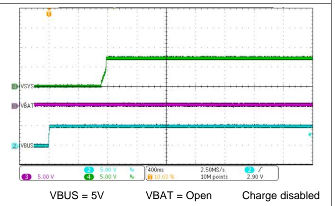
Figure 81. Adapter Plug-in with No Dead Battery
