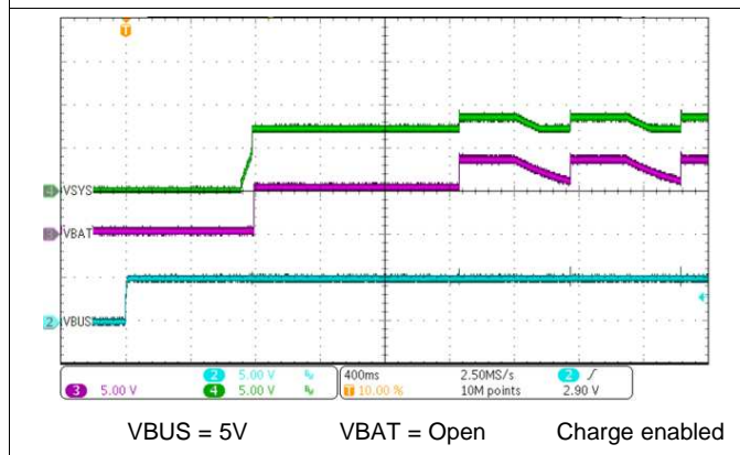
Figure 80. Adapter Plug-in with No Battery
