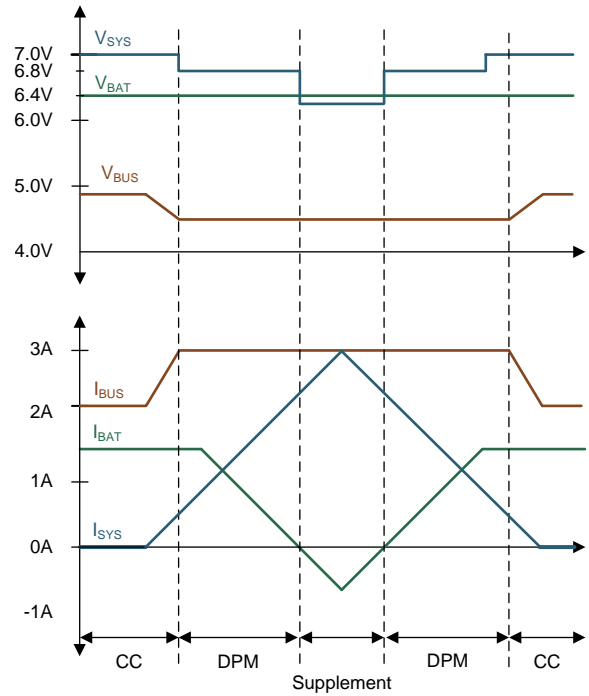
Figure 20. DPM Response
