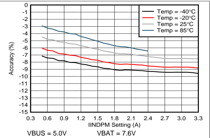
Figure 14. Input Current Limit Accuracy vs. IINDPM Setting
