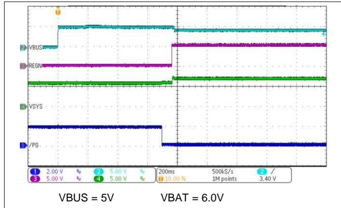
Figure 76. Adapter Power Up With Charge Enabled
