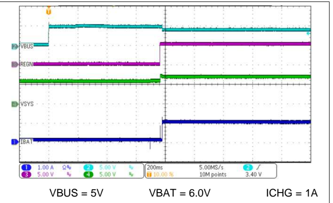
Figure 77. Adapter Power Up With Charge Enabled
