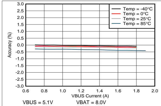
Figure 13. OTG Voltage Regulation vs. OTG BUS Current
