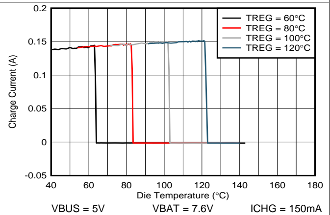
Figure 16. TREG Profiles
