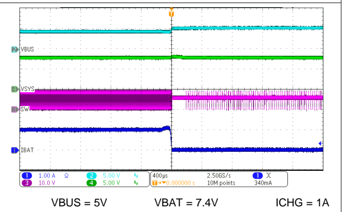
Figure 79. Charge Disable
