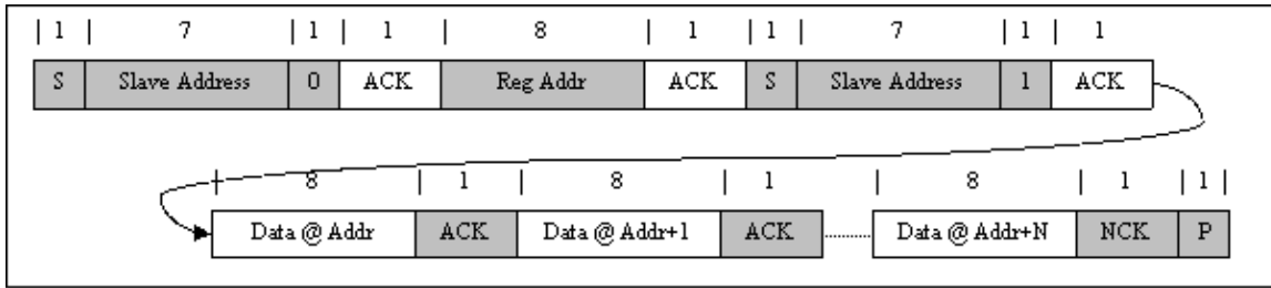
Figure 35. Multi-Read
