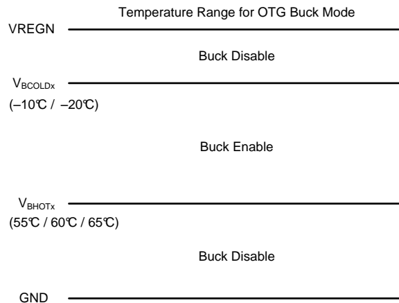
Figure 25. TS Pin Thermistor Sense Threshold in OTG Buck Mode
