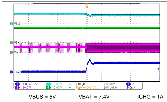
Figure 78. Charge Enable
