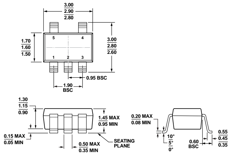
COMPLIANT TO JEDEC STANDARDS MO-178-AA Figure 69. 5-Lead Small Outline Transistor Package [SOT-23] (RJ-5)
