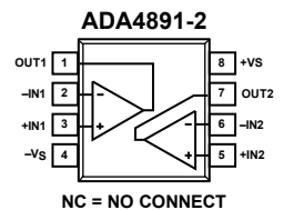
Figure 3. 8-Lead SOIC N (R-8) and 8-Lead MSOP (RM-8)
