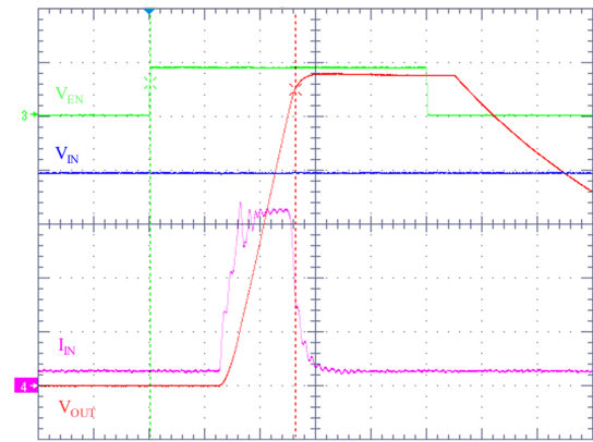
Figure 27. Inrush current
