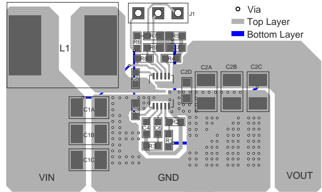
Figure 5: Layout Recommendation
