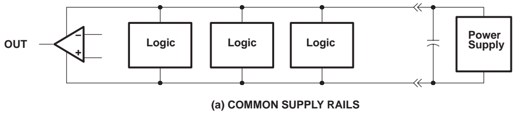
(a) COMMON SUPPLY RAILS
