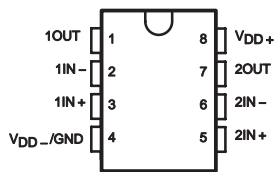
TLV2252I, TLV2252AI TLV2252Q, TLV2252AQ D, P, OR PW PACKAGE (TOP VIEW)
