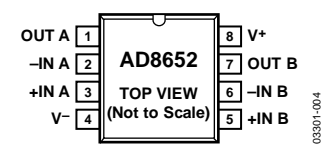
Figure 4. 8-Lead SOIC_N (R-8)
