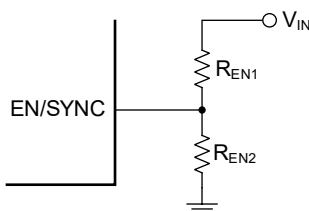
Figure 3. EN Resistor Divider
