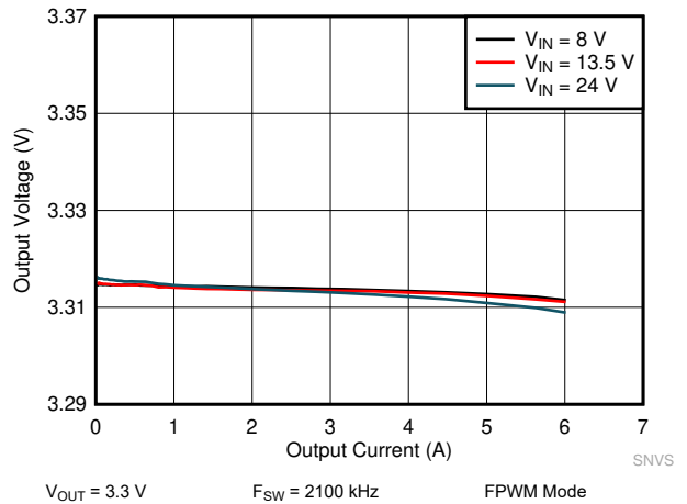
Figure 10-16. LM61460-Q1 Load and Line Regulation
