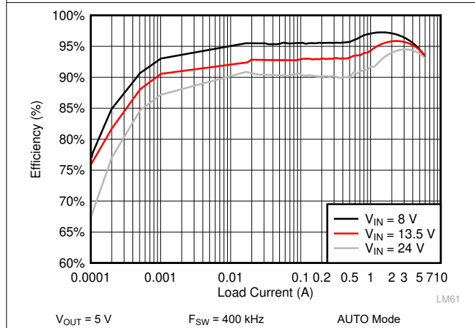
Figure 10-9. LM61460-Q1 Efficiency
