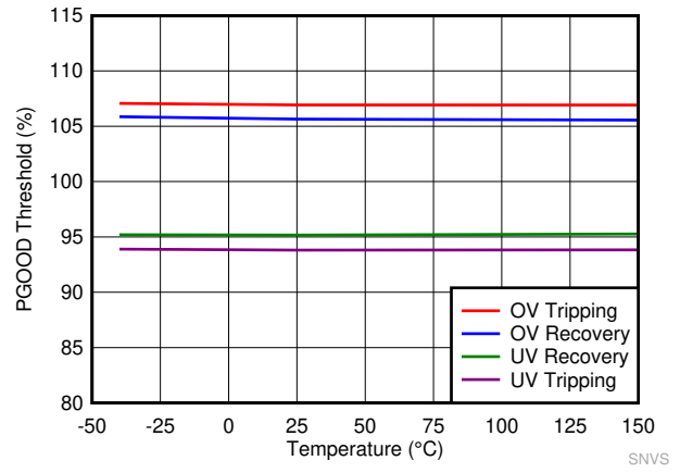
Figure 8-8. PGOOD Thresholds
