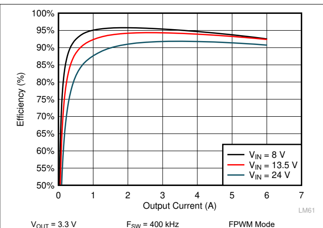
Figure 10-6. LM61460-Q1 Efficiency
