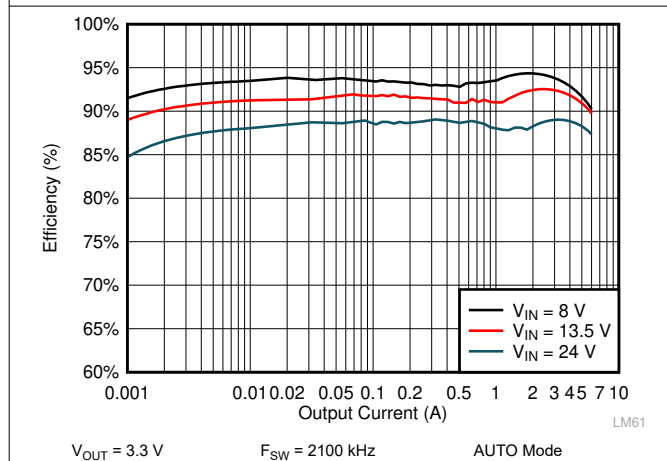
Figure 10-7. LM61460-Q1 Efficiency
