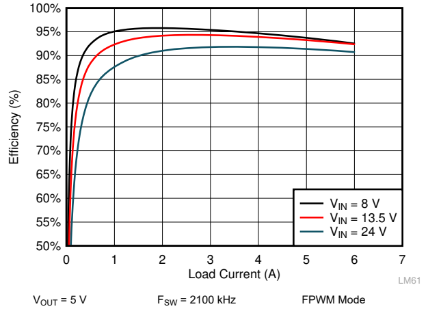
Figure 10-12. LM61460-Q1 Efficiency
