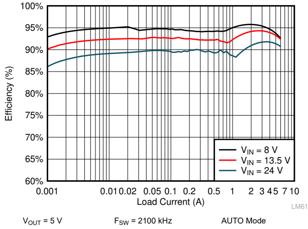
Figure 10-11. LM61460-Q1 Efficiency
