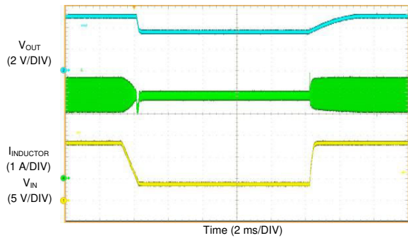
Figure 10-35. LM61460-Q1 Short Circuit Recovery
