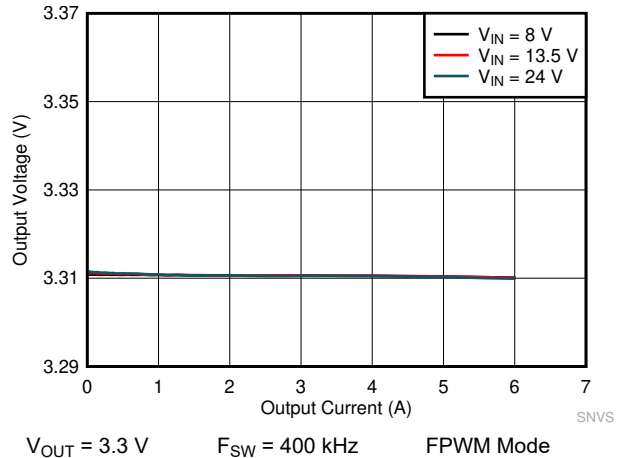
Figure 10-14. LM61460-Q1 Load and Line Regulation
