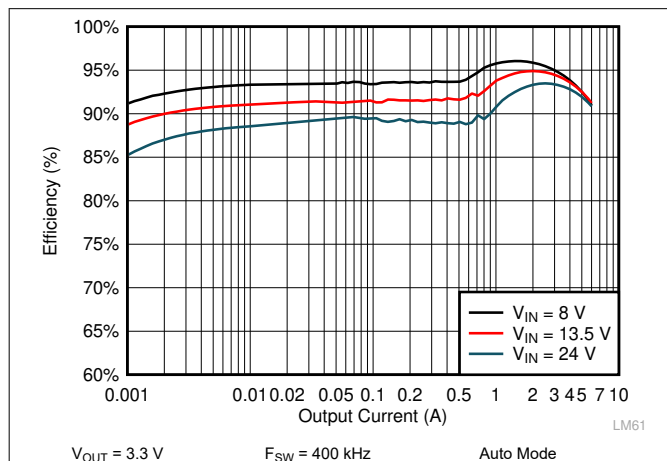
Figure 10-5. LM61460-Q1 Efficiency
