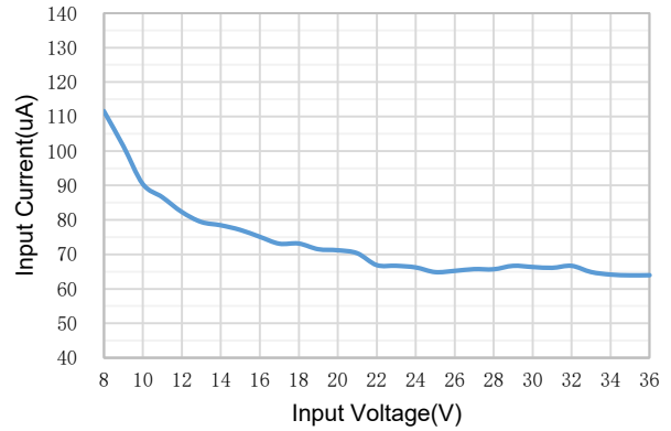
Figure 5. Input Current ( V_{out}=5V , I_{load}=0A )
