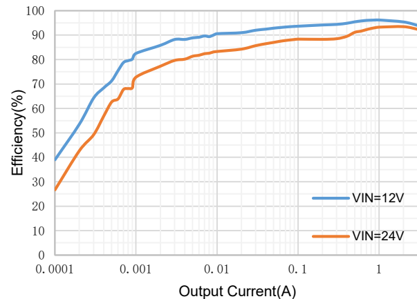
Efficiency, V_{OUT}=5V , F_{sw}=400KHz
