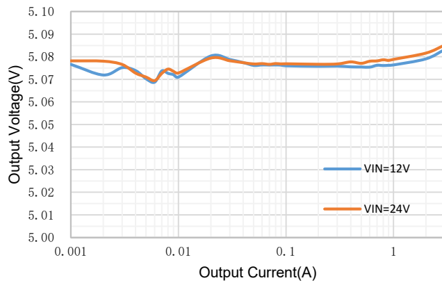
Figure 6. Load Regulation ( V_{out}=5V )
