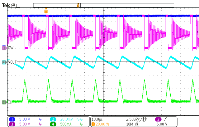
Figure 20. Output Ripple ( I_{LOAD}=100mA )
