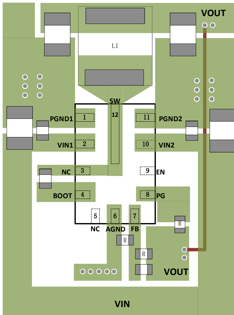
Figure 24. PCB Layout Example
