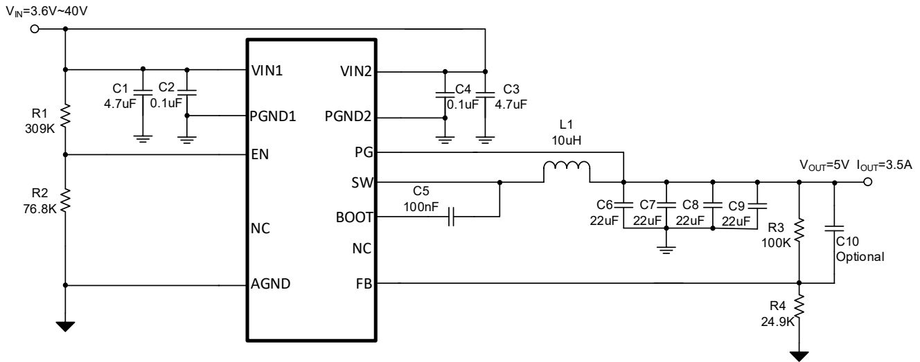
Figure 11. SCT2434A Design Example, 5V Output with Adjustable UVLO
