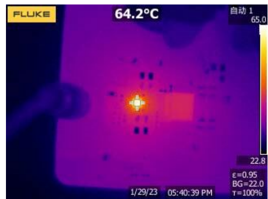
Figure 23. Thermal, 12VIN, 5VOUT, 3.5A
