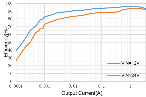
Figure 3. Efficiency, F_{sw}=400KHz , V_{out}=5V
