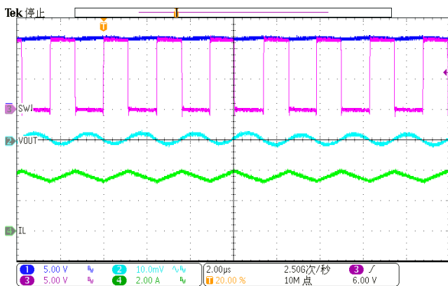
Figure 22. Output Ripple ( I_{LOAD}=3.5A )
