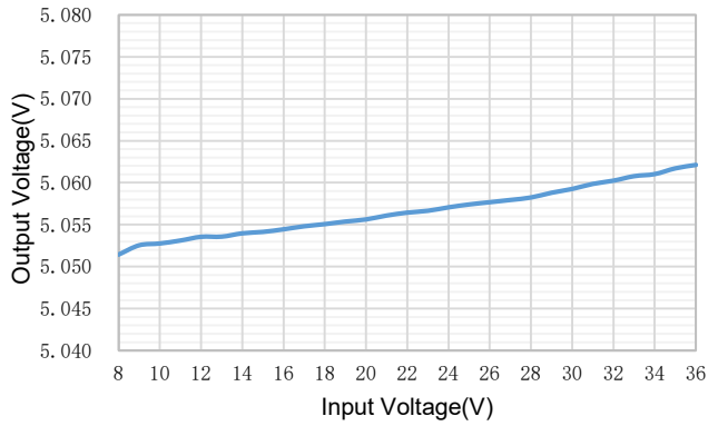
Figure 4. Line Regulation ( V_{out}=5V , I_{load}=3.5A )
