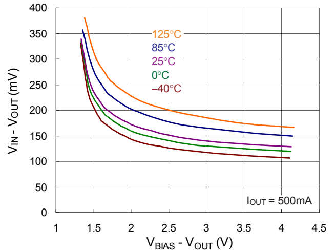
V IN Dropout Voltage vs. (V BIAS - V OUT )
