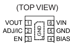
ZADFN-6L 1.2x1.2
