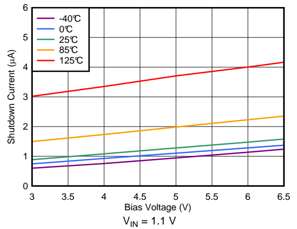
Figure 38. Shutdown Current vs Bias Voltage
