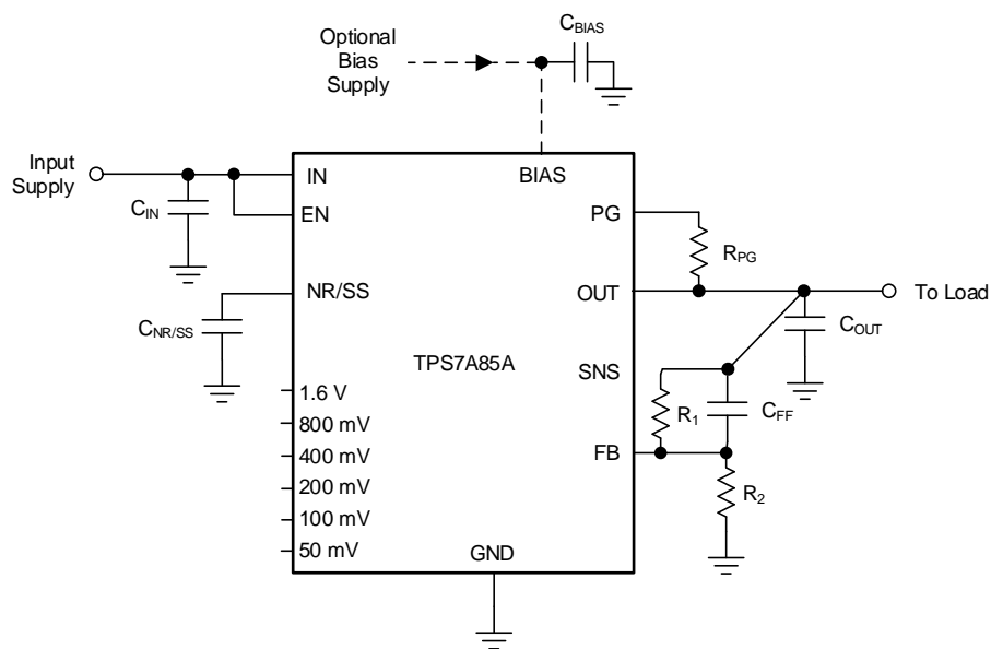
Figure 50. Adjustable Operation
