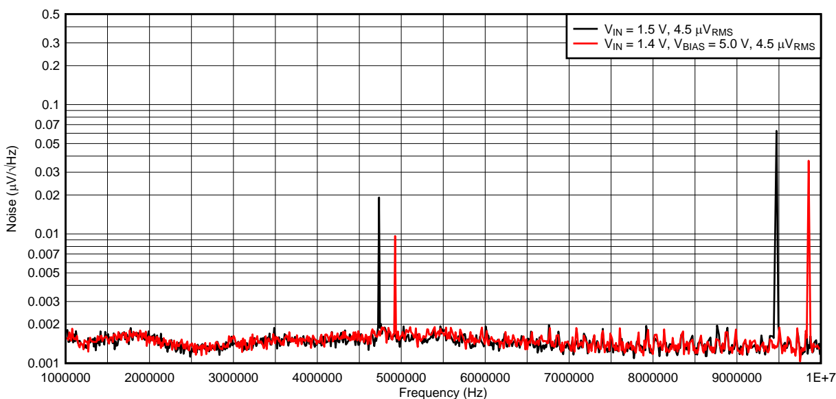
Figure 57. Charge Pump Noise
