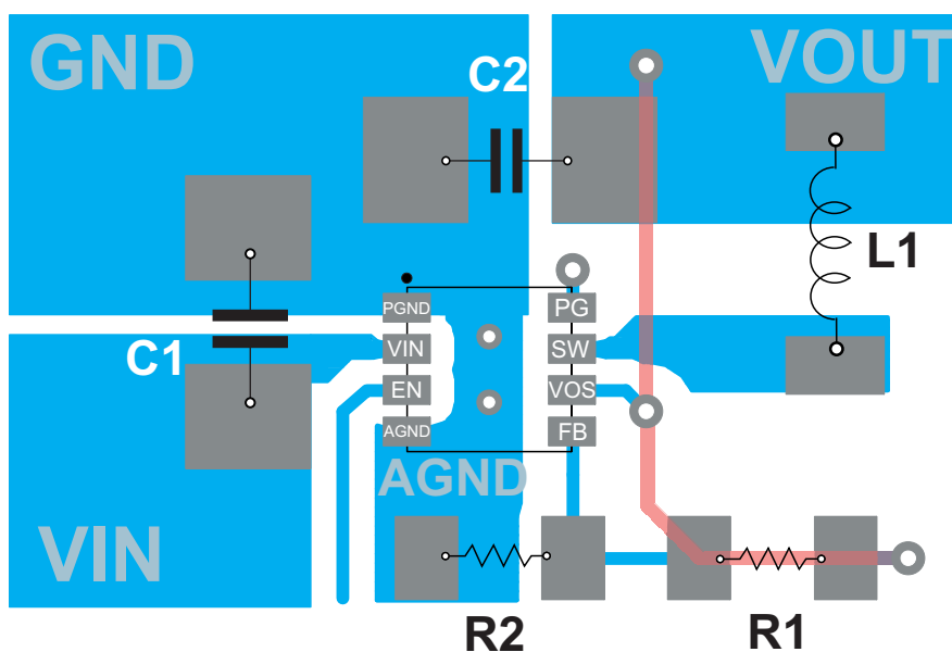
Figure 38. Layout Example
