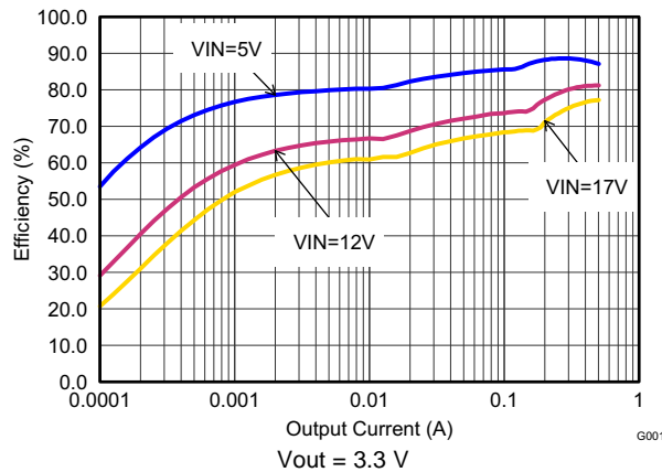
Figure 9. Efficiency versus Input Voltage
