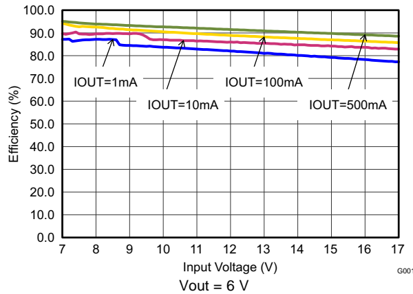
Figure 7. Efficiency versus Input Voltage
