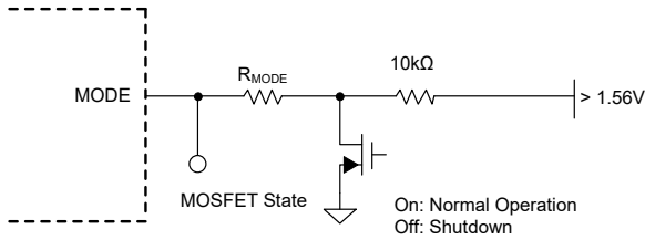
Figure 5. Shutdown in Frequency Adjustment Mode
