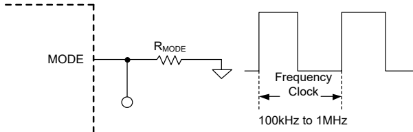
Figure 4. Frequency Synchronization
