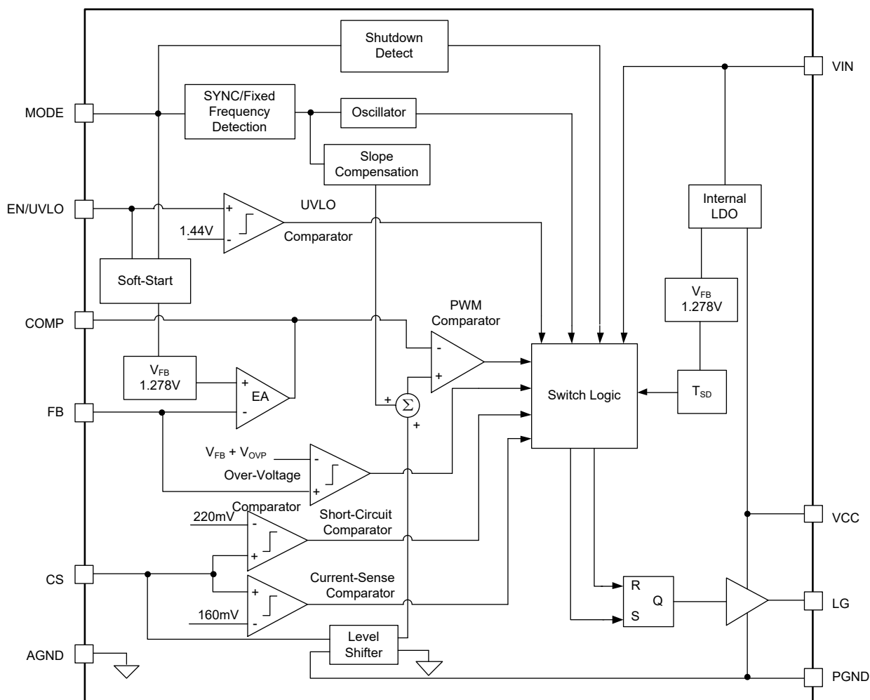
Figure 2. Block Diagram
