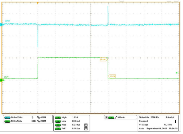
Figure 27. Load transient
