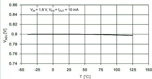
Figure 4. V_{ADJ} accuracy
