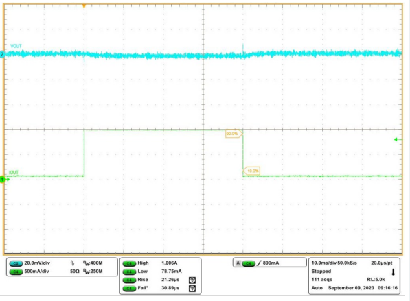
Figure 25. Load transient
