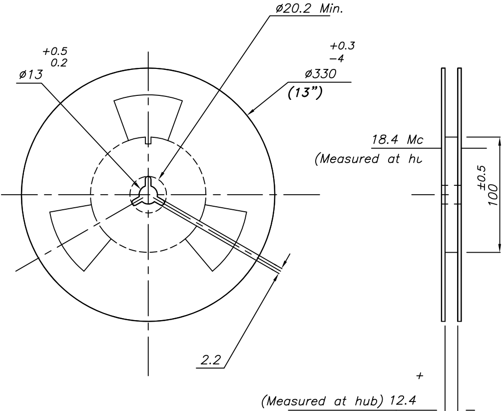
Figure 36. DFN6 (3x3 mm) reel outline
