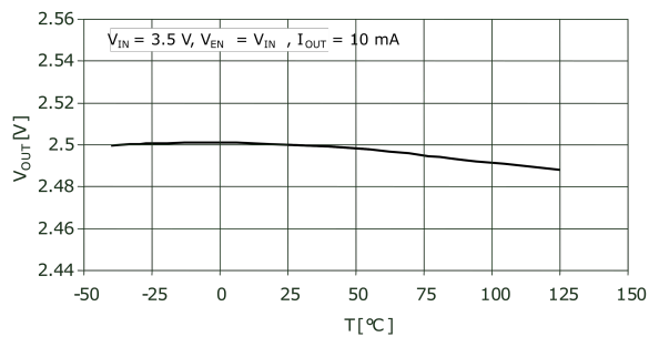
Figure 5. V_{OUT} accuracy
