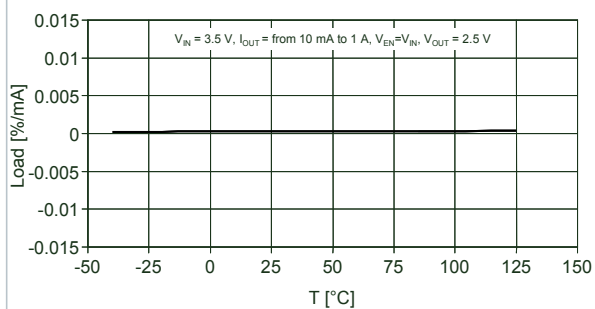
Figure 14. Load regulation
