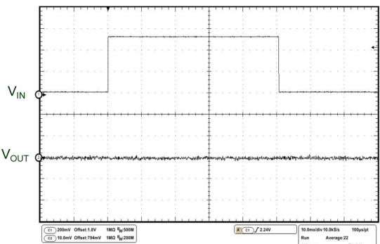
Figure 23. Line transient
