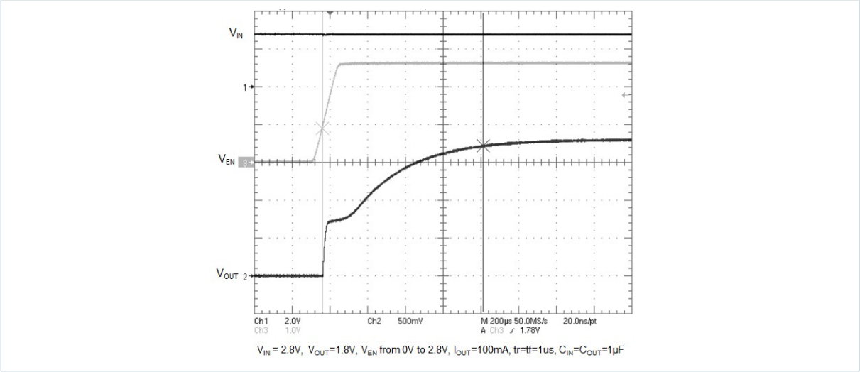
Figure 28. Enable transient
