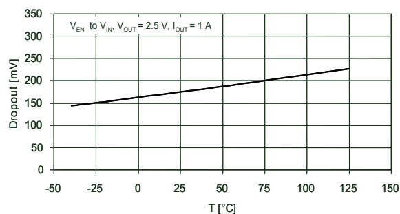
Figure 6. Dropout voltage vs. temperature ( V_{OUT} = 2.5 V)
