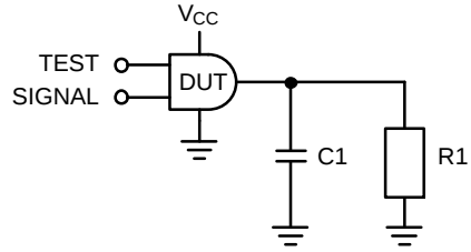
Figure 2. Test Circuit
