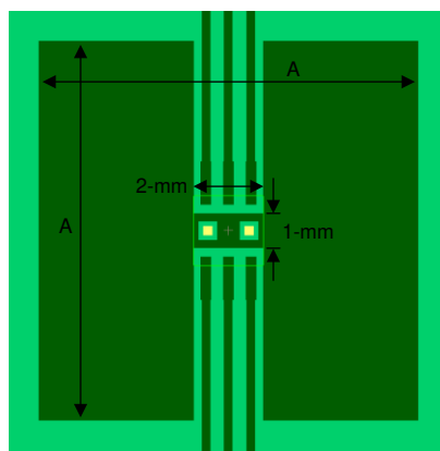
Figure 8-7. Board parameters used for simulation
