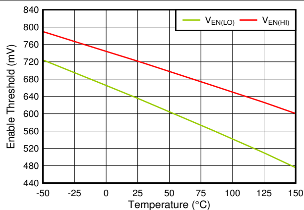
Figure 6-27. V_{EN(HI)} and V_{EN(LO)} vs Temperature
