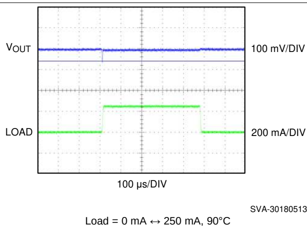
Figure 12. Load Transient
