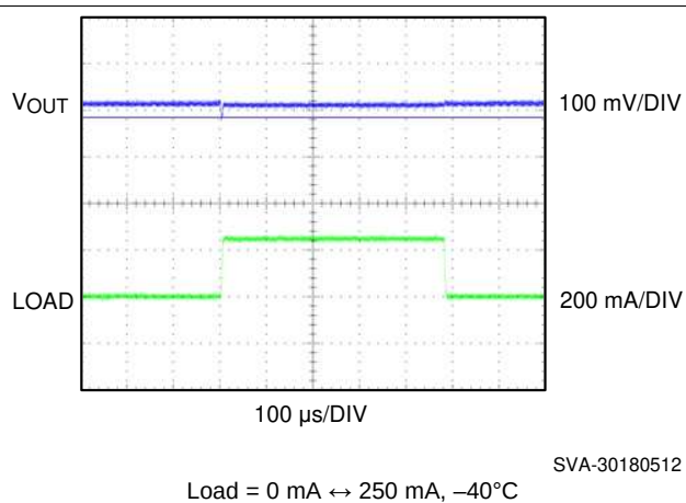
Figure 11. Load Transient
