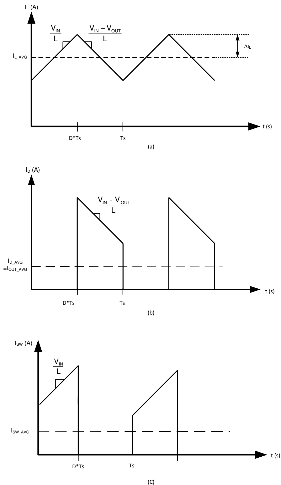
Figure 7-3. Inductor Current and Diode Current
