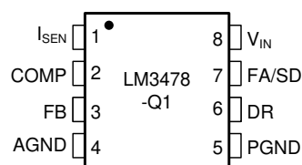
Figure 4-1. LM3478-Q1 DKG Package, VSSOP-8 (Top View)
