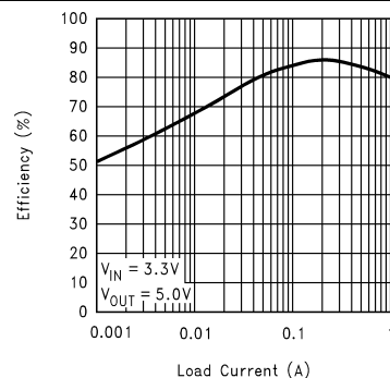
Figure 7-7. Efficiency vs Load Current (3.3-V In and 5-V Out)
