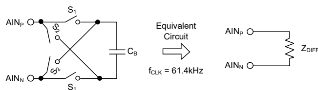
Figure 7. Simplified Analog Input Circuit
