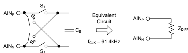
Figure 6. Simplified Analog Input Circuit
