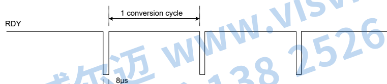
Figure 9. RDY in Continuous Mode
