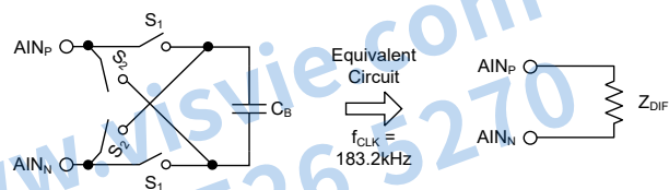
Figure 5. Simplified Analog Input Circuit
