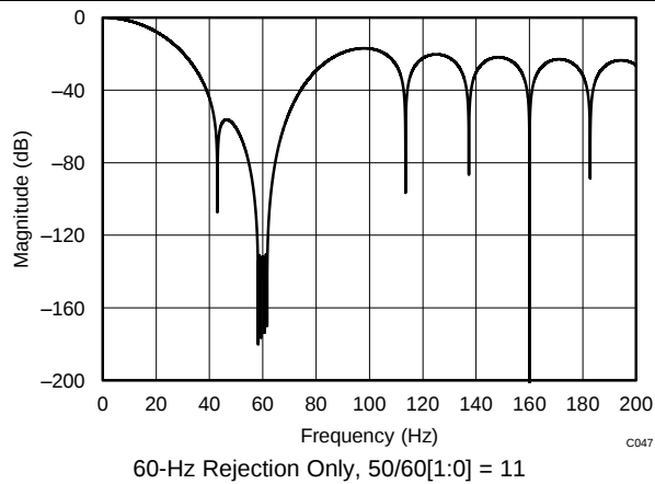
Figure 50. Filter Response (DR = 20 SPS)
