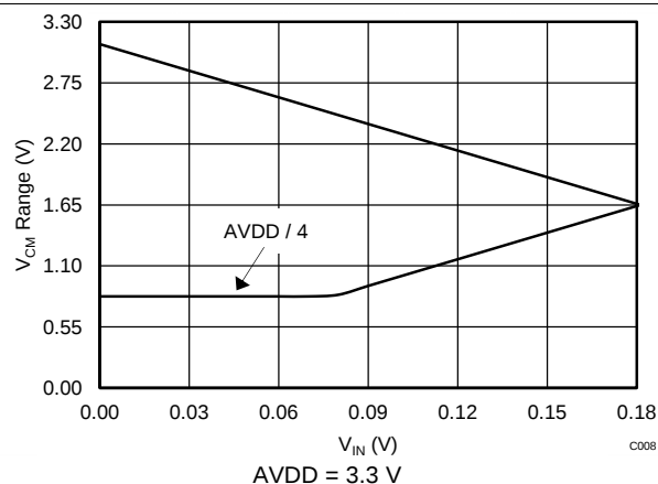
Figure 42. Common-Mode Voltage Limits (Gain = 16)
