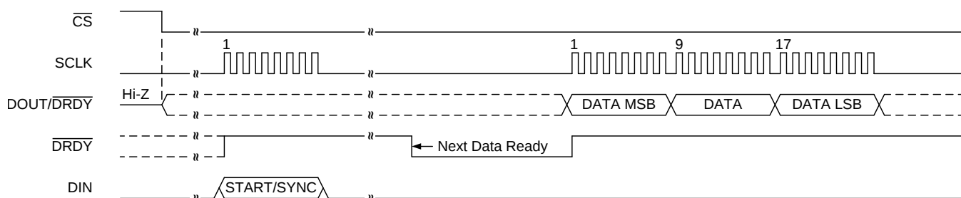
Figure 63. Single-Shot Mode ( \overline{\text{DRDYM}} = 0 )
