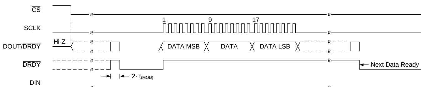
Figure 62. Continuous Conversion Mode ( \overline{\text{DRDYM}} = 1 )
