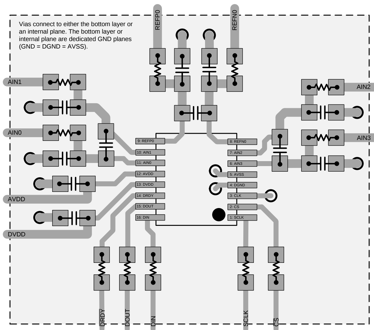
Figure 87. Layout Example
