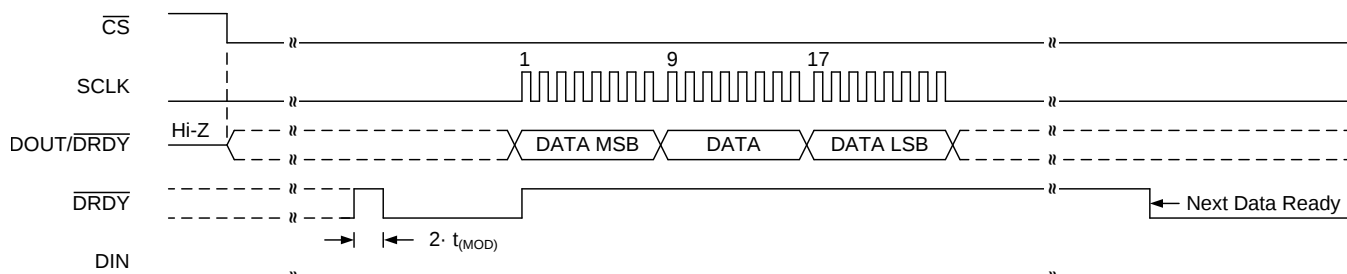
Figure 61. Continuous Conversion Mode ( \overline{\text{DRDYM}} = 0 )
