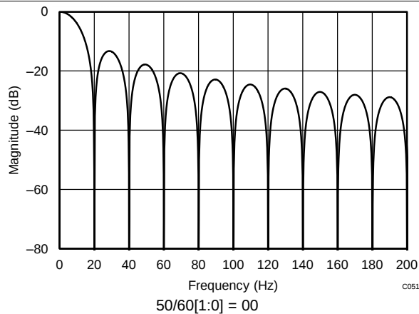
Figure 52. Filter Response (DR = 20 SPS)
