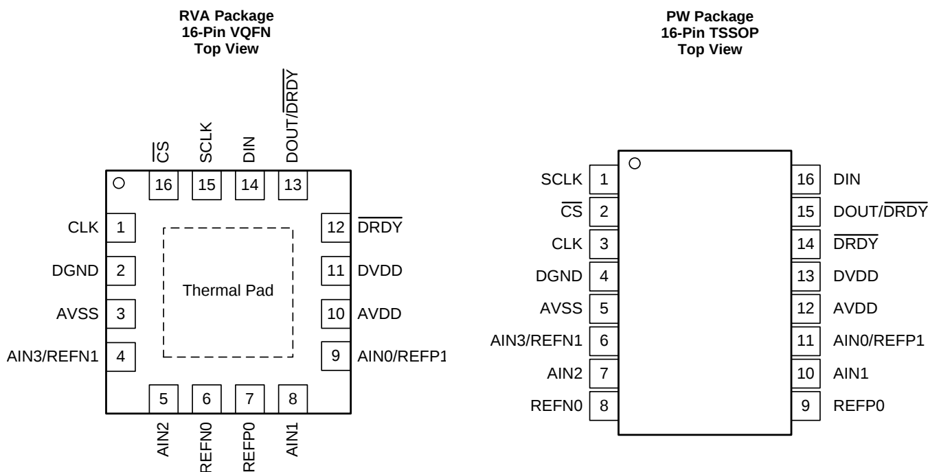
Pin Functions
