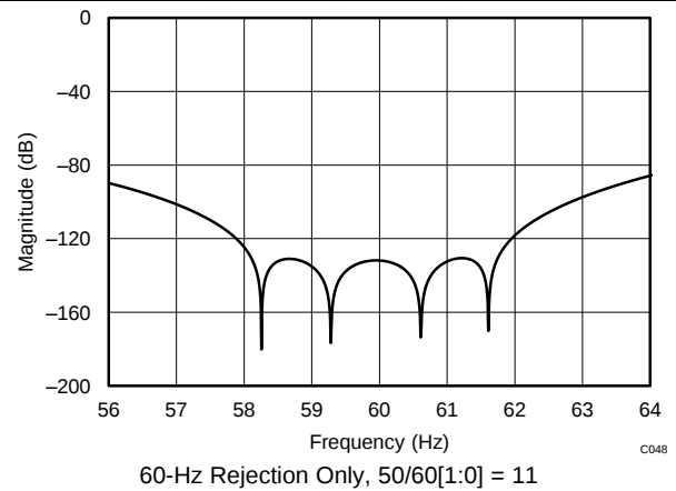
Figure 51. Detailed View of Filter Response (DR = 20 SPS)
