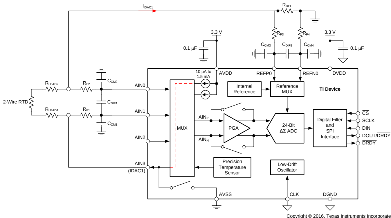
Figure 78. 2-Wire RTD Measurement
