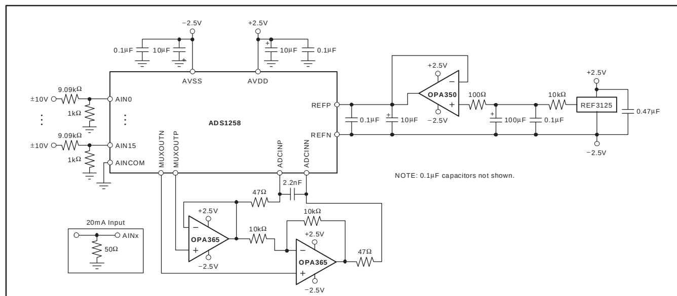
Figure 67. Multichannel, \pm 10\text{V} Single-Ended Input, Bipolar Supply Operation
