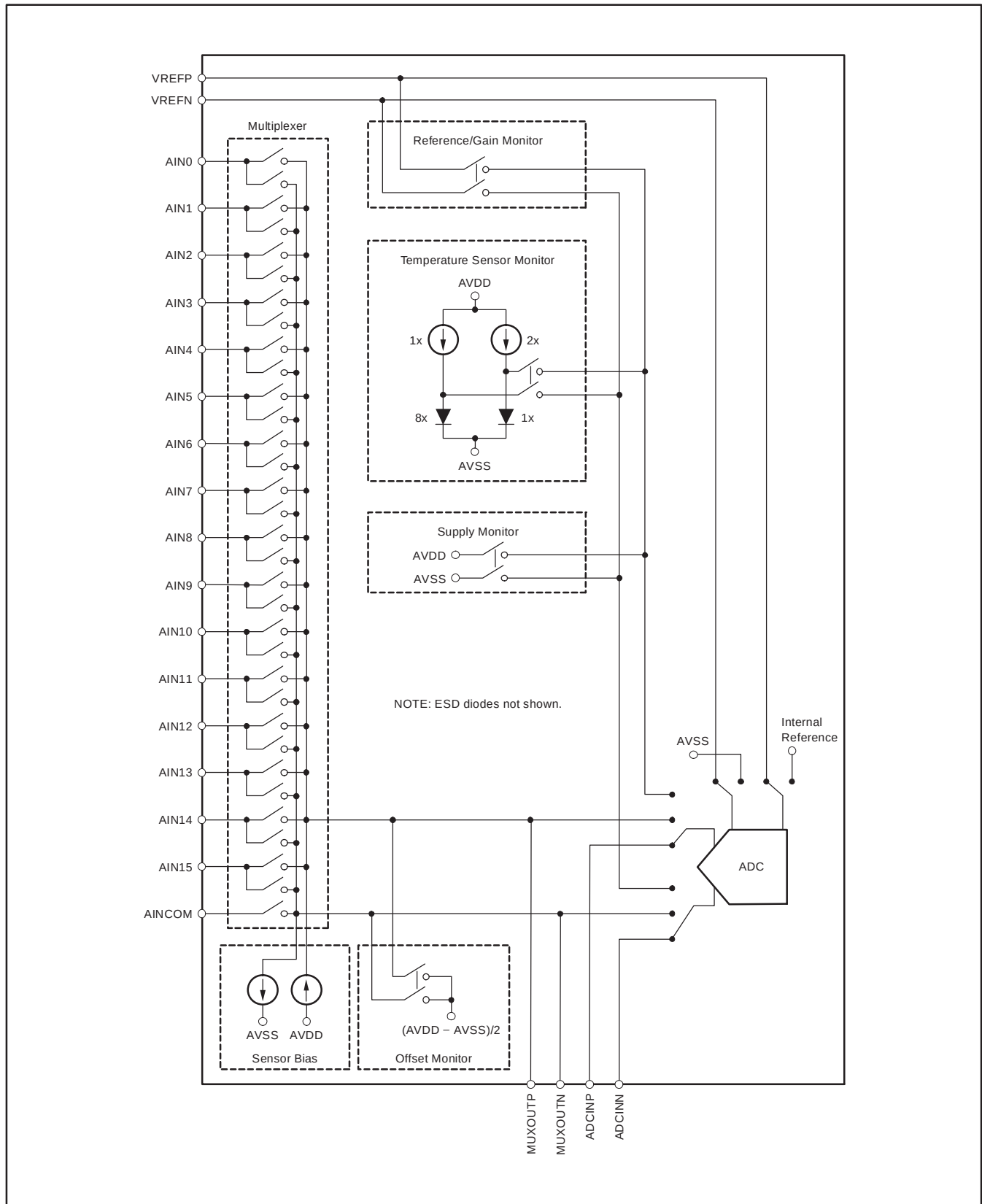
Figure 35. Input Multiplexer
