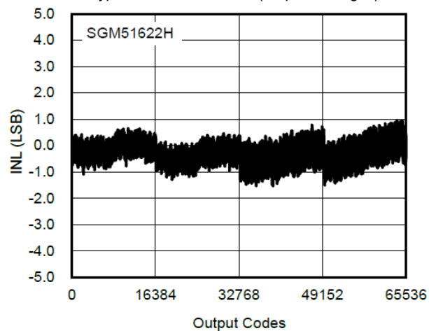
Typical INL for All Codes (Unipolar Ranges)
