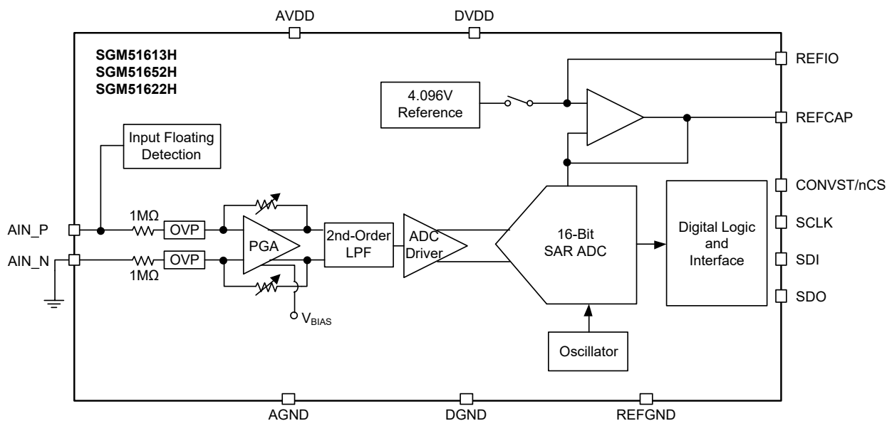
Figure 5. Block Diagram
