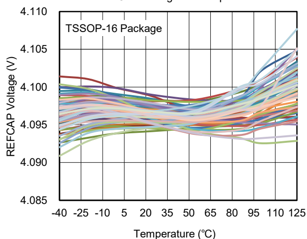
REFCAP Voltage vs. Temperature
