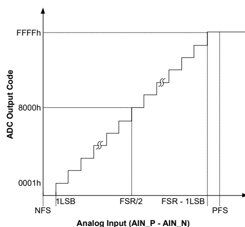
Figure 8. Device Transfer Function (Straight-Binary Format)
