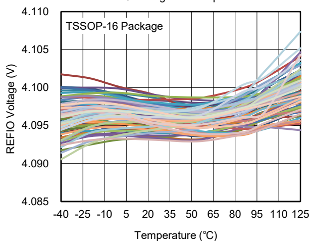
REFIO Voltage vs. Temperature
