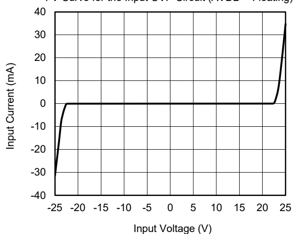
I-V Curve for the Input OVP Circuit (AVDD = Floating)
