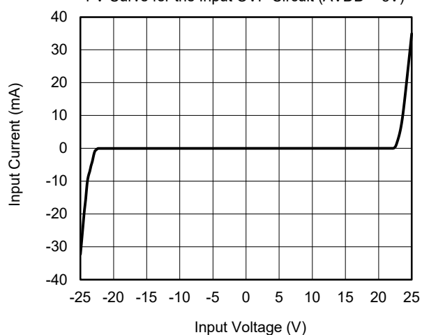
I-V Curve for the Input OVP Circuit (AVDD = 5V)
