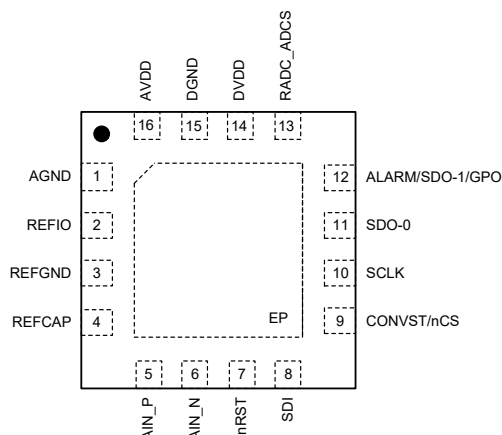
TQFN-4x4-16L
