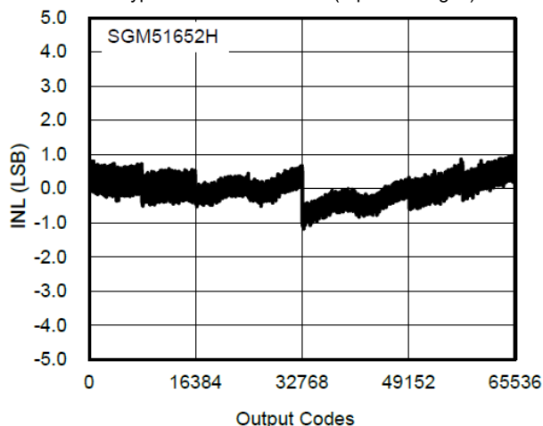
Typical INL for All Codes (Bipolar Ranges)
