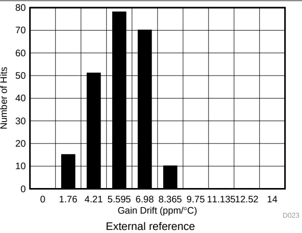
Figure 27. Gain Error Drift Histogram Distribution ( \pm 10\text{ V} )
