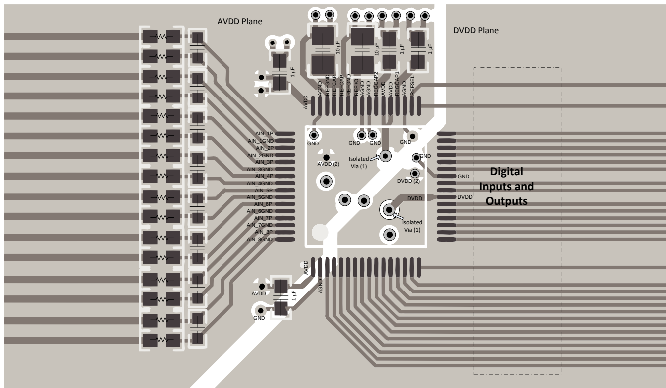
Figure 89. Top Layer Layout
