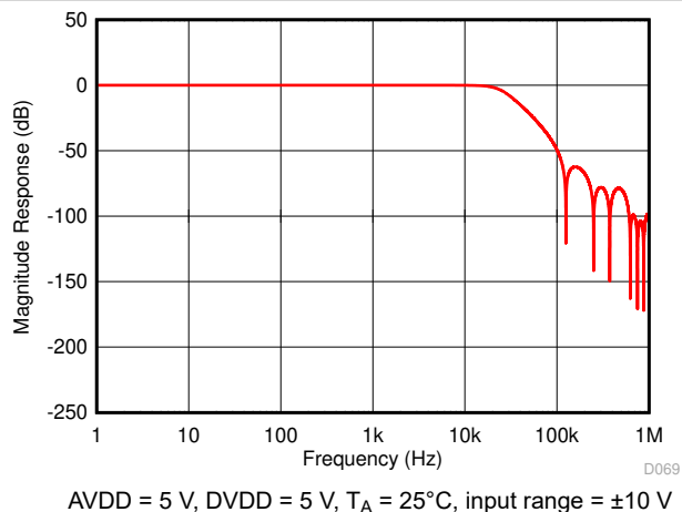
Figure 7-28. Digital Filter Response for OSR = 4
