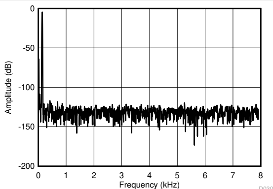
Figure 6-34. Typical FFT Plot for OSR 32x ( \pm 10\text{ V} )
