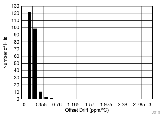
Figure 6-22. Offset Drift Histogram Distribution ( \pm 10\text{ V} )
