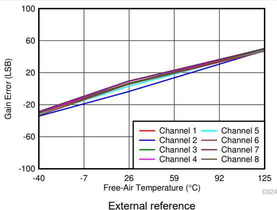
Figure 6-28. Gain Error Across Channels vs Free-Air Temperature ( \pm 10\text{ V} )
