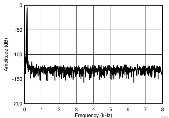
Figure 6-35. Typical FFT Plot for OSR 32x ( \pm 5\text{ V} )
