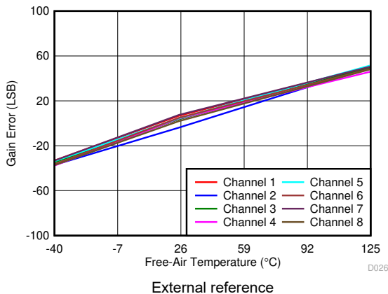
Figure 6-30. Gain Error Across Channels vs Free-Air Temperature ( \pm 5\text{ V} )
