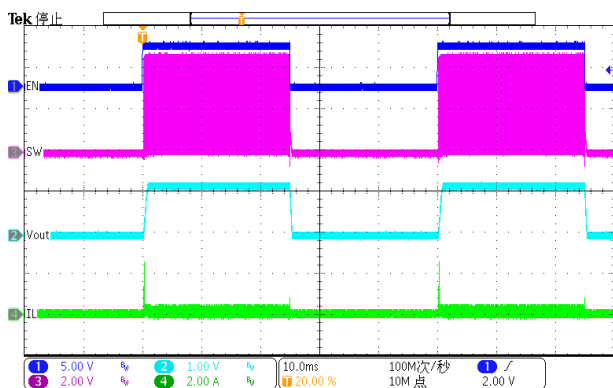
Figure 11. EN toggle ( I_{LOAD}=0.1A )
