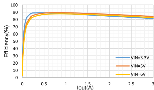
Efficiency, Vout=1.2V
