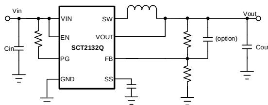
2.8V-6V, Synchronous Buck Converter
