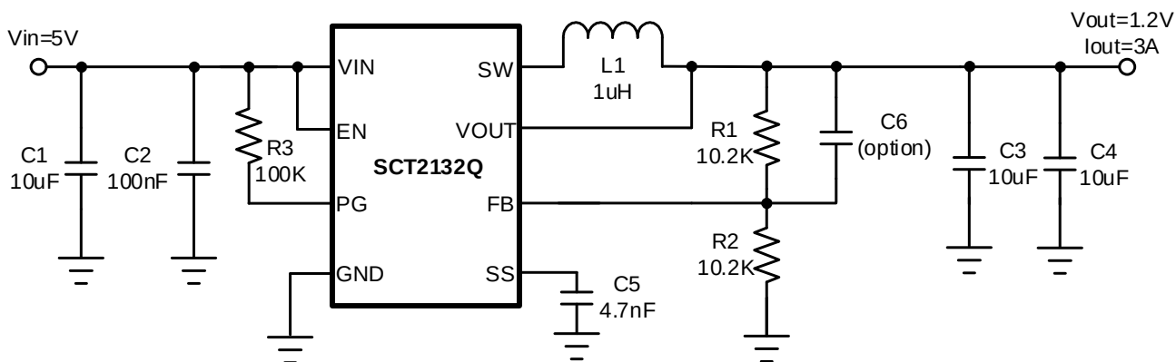
Figure 8. SCT2132Q Design Example, 1.2V Output
