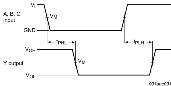
Fig. 4. The input (A, B, C) to output (Y) propagation delays
