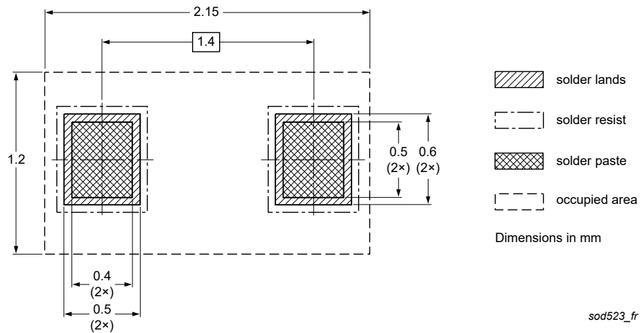
Fig. 10. Reflow soldering footprint for SC-79 (SOD523)
