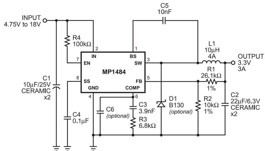
Figure 3—MP1484 with 3.3V Output, 22uF/6.3V Ceramic Output Capacitor
