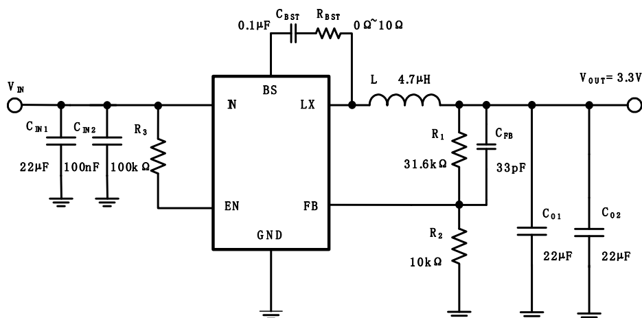
Figure 1. EUP3163 Typical Application Circuits
