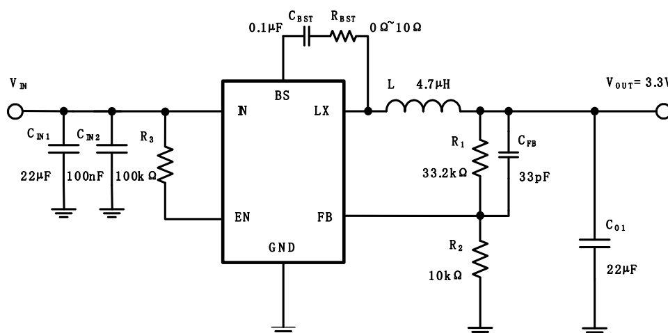
Figure 1. EUP3132 Typical Application Circuits
