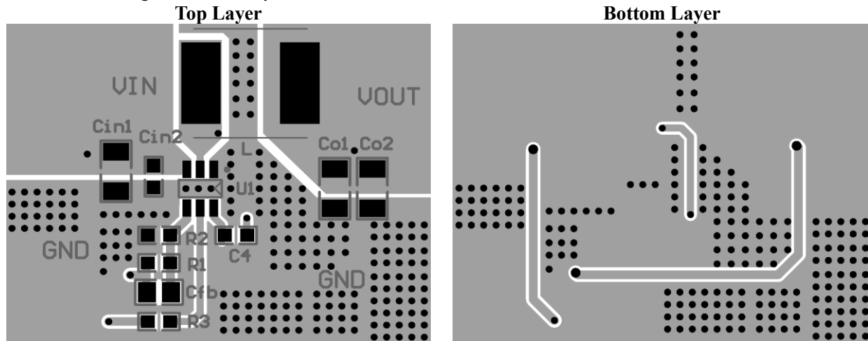
Figure 4. Sample of PCB Layout (EUP3132)
