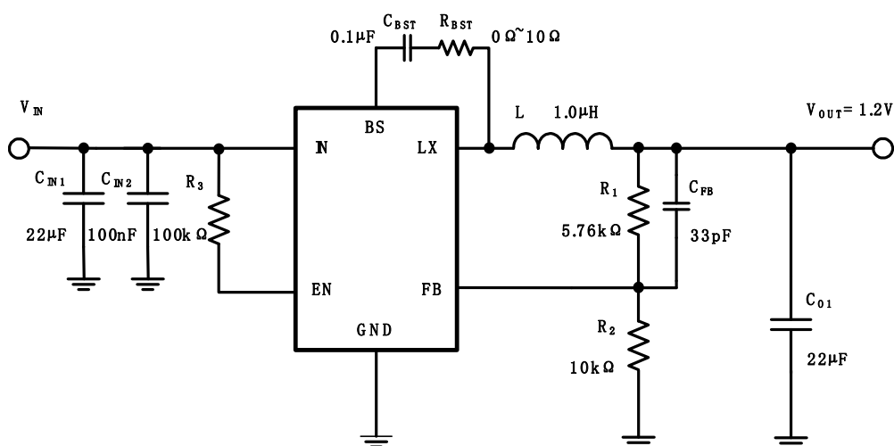
Figure 9. Application Circuits of 12V Input, 1.2V Output
