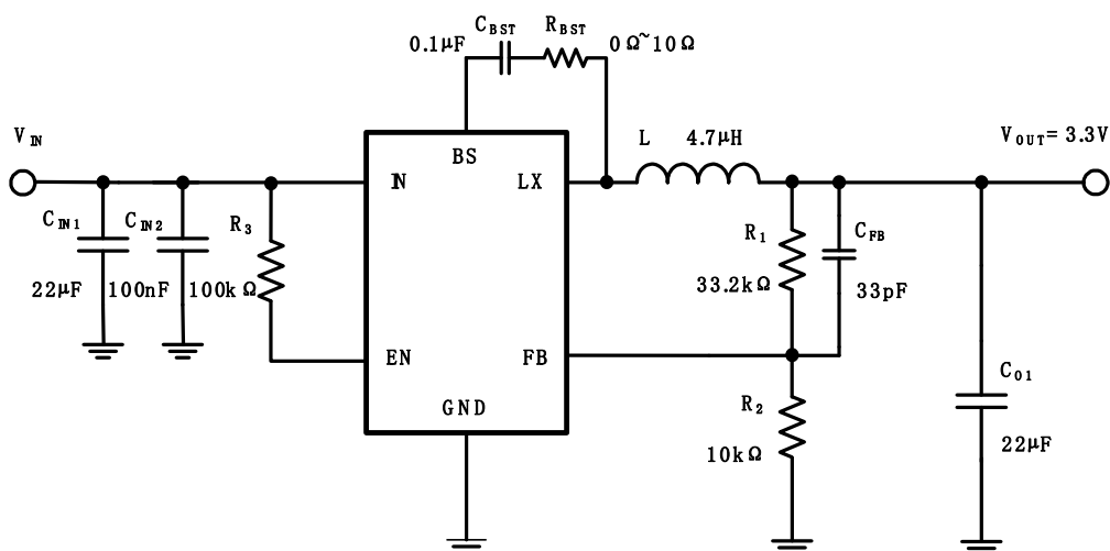
Figure 6. Application Circuits of 12V Input, 3.3V Output
