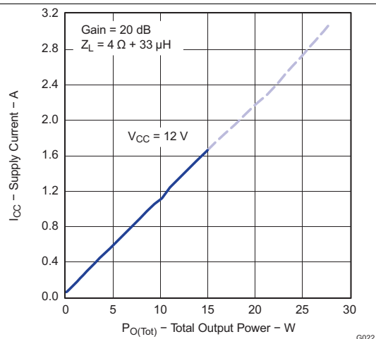
Figure 26. Supply Current vs Total Output Power (BTL)
