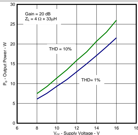
Figure 18. Output Power vs Supply Voltage (BTL)
