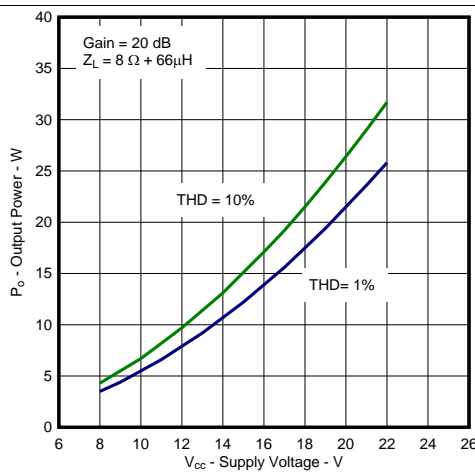
Figure 16. Output Power vs Supply Voltage (BTL)
