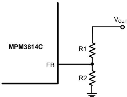
Figure 2: Feedback Network
