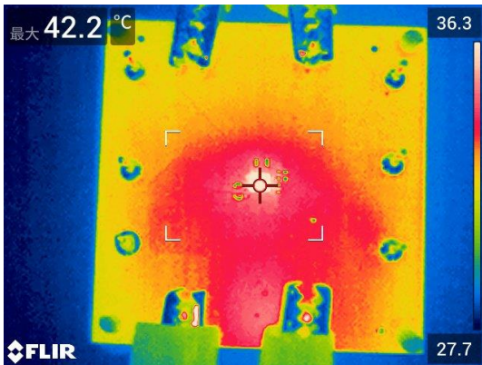
Thermal Result I_{OUT} = 1A , 4-layer PCB
